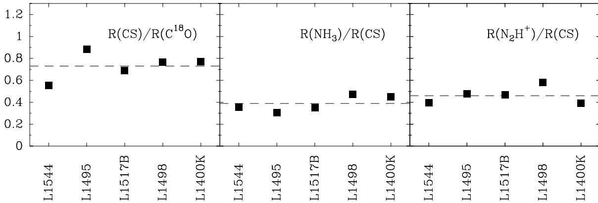
FIG. 8.— Ratio of map sizes (half-maximum radius) for different molecules as measured from the best-fit Monte Carlo models represented in Figs. 3, 5, and 6. The dashed lines represent the mean value for each molecular pair (see text). Note how the \text{NH}_3 sizes are systematically smaller than the CS sizes by a factor larger than 2. This systematic size discrepancy, already known but unexplained, is a consequence of the central abundance drop of CS, which severely truncates the emission from this molecule and therefore increases the half-maximum radius. See text for a complete discussion.
